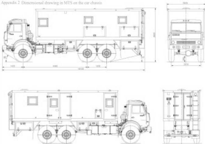
Appendix 2 Dimensional drawing in MTS on the car chassis
